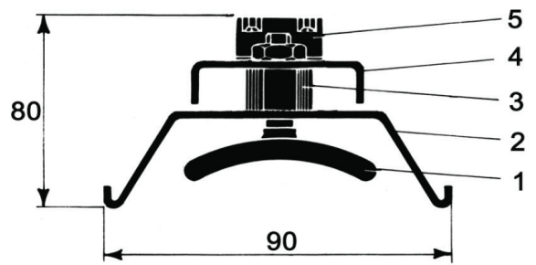
Reflector Assemblies
